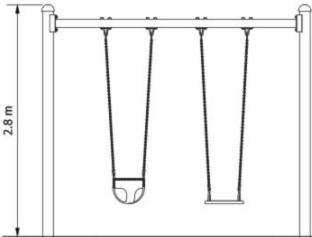
SOUTH-EAST ELEVATION
