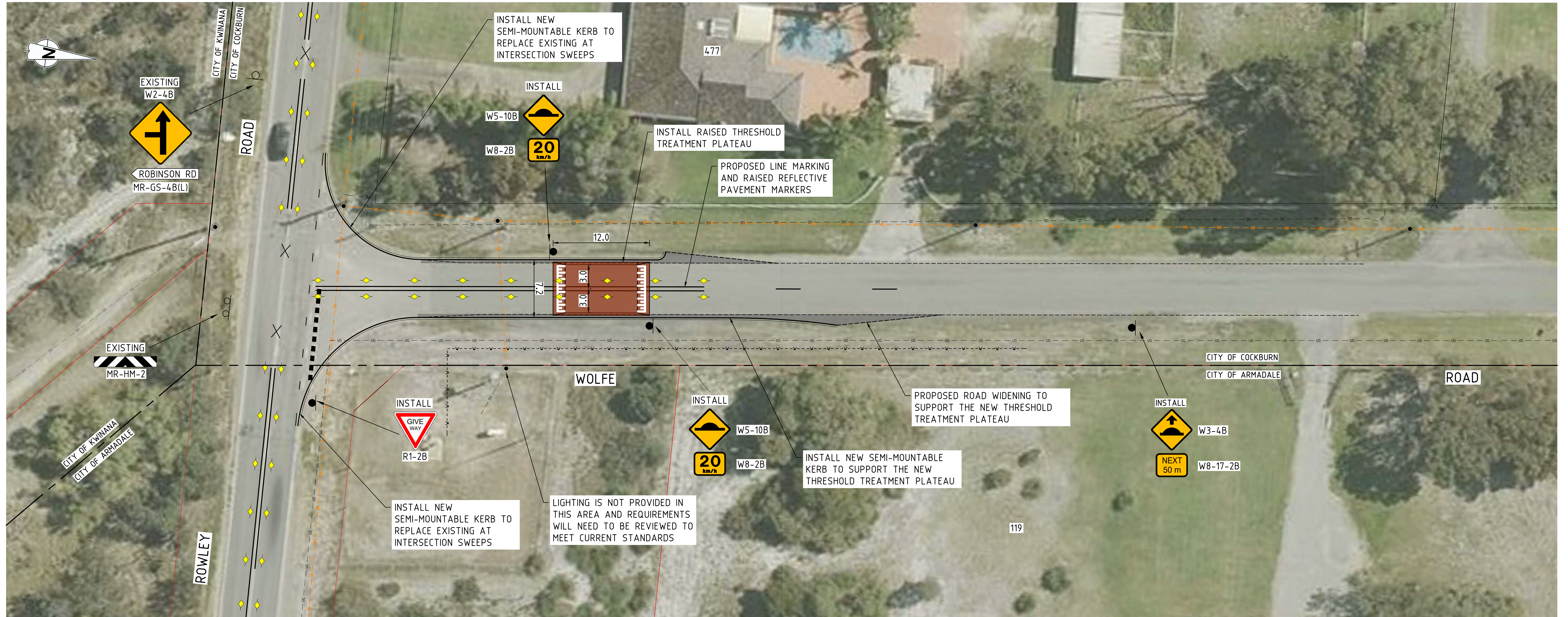
PLAN SCALE 1:250
