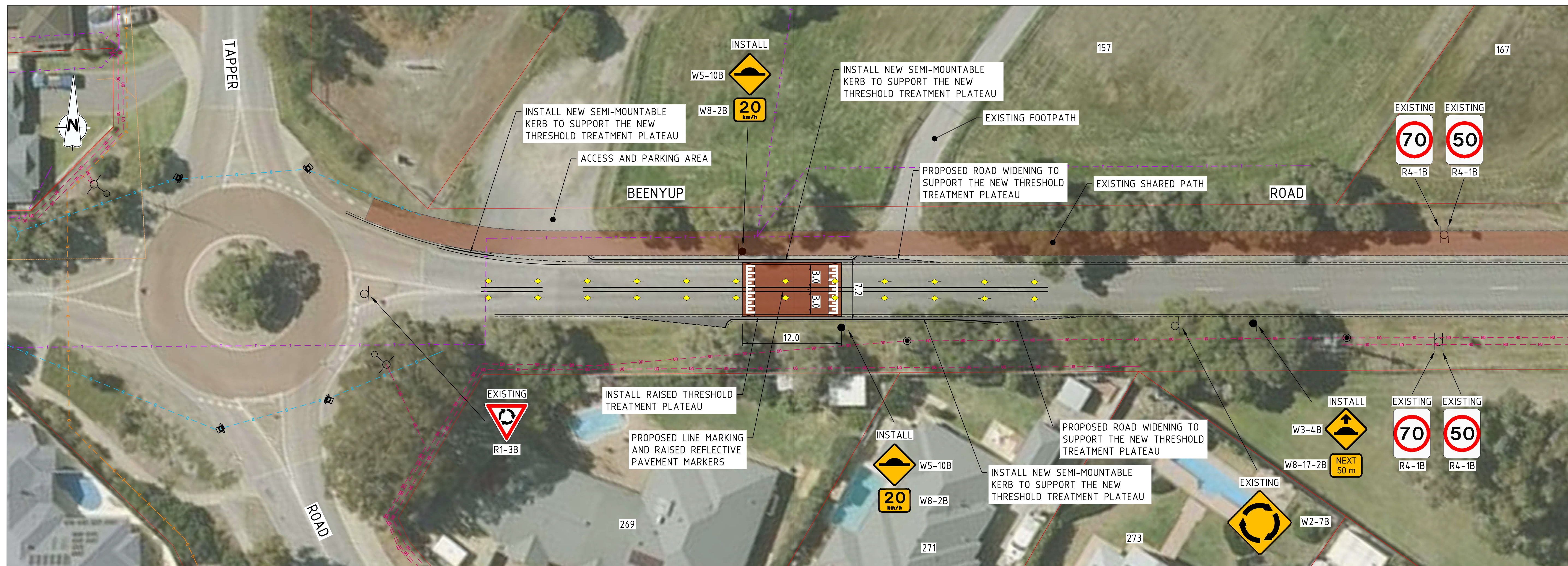
PLAN SCALE 1:250
