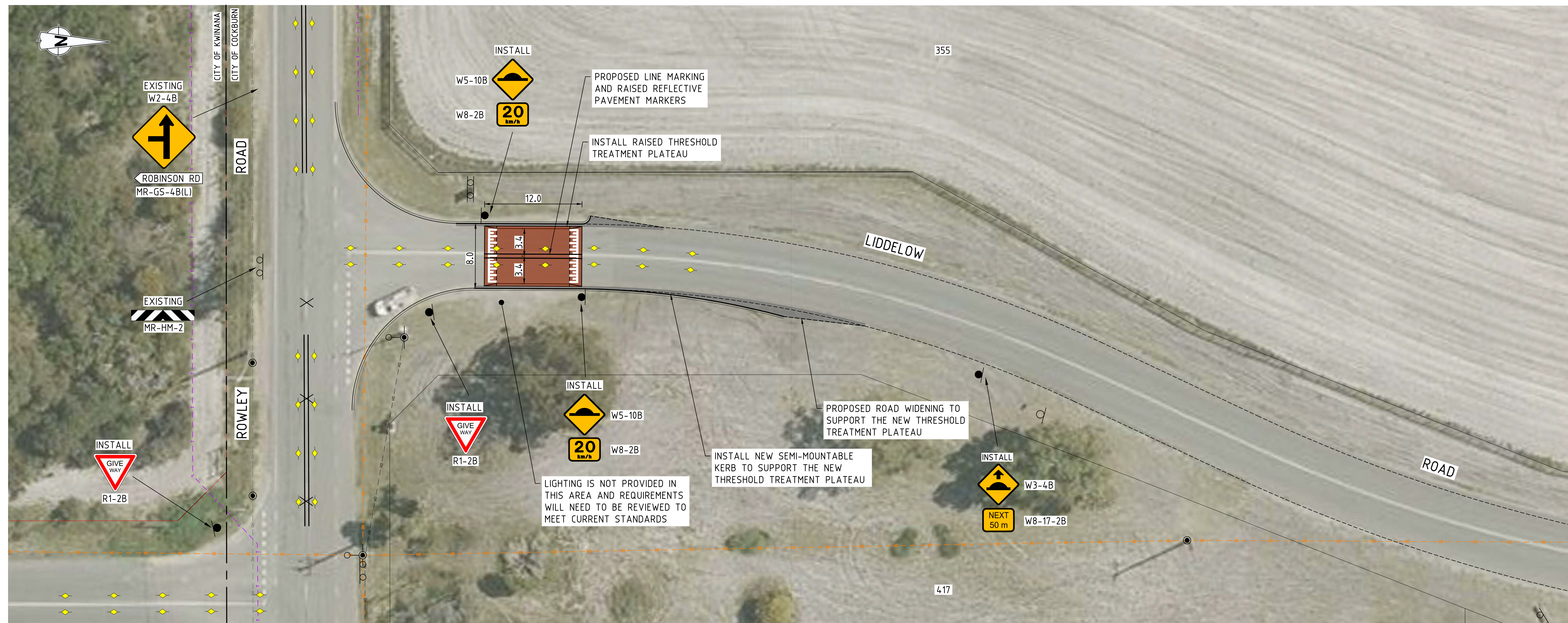
PLAN SCALE 1:250
