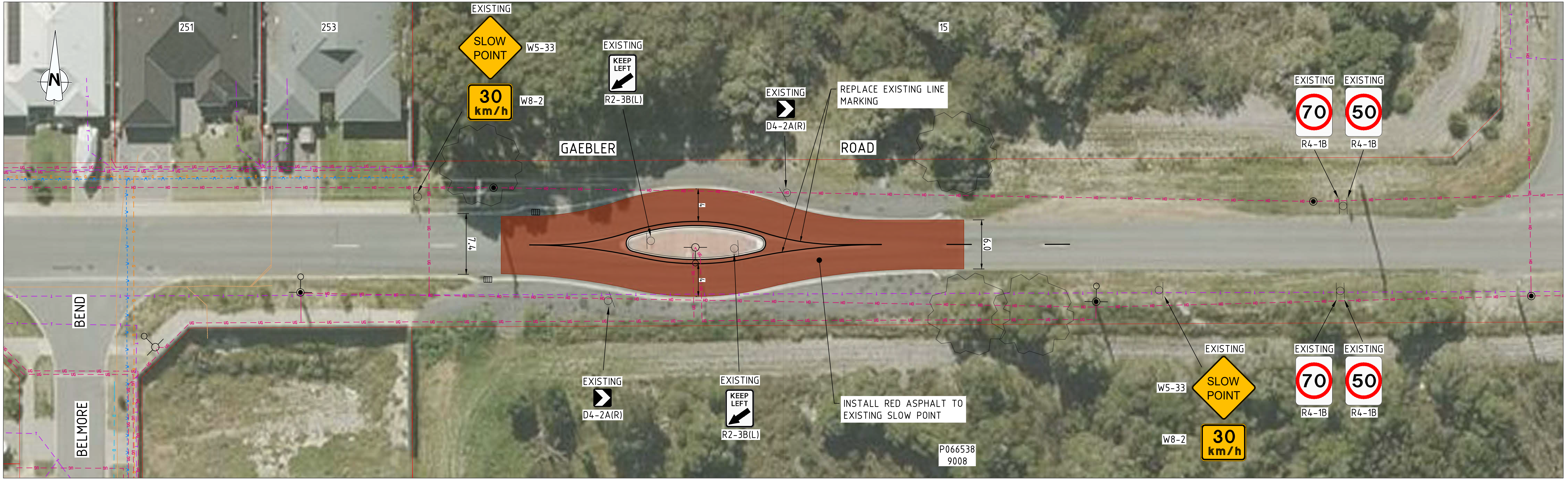
PLAN SCALE 1:250
